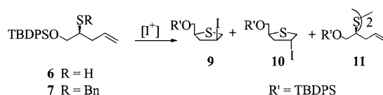
Scheme 4. Iodine-induced cyclization of 2-sulfanyl-4-penten-1-ol derivatives
