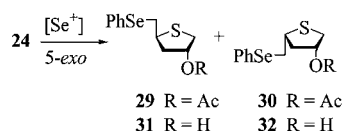
Scheme 8. Selenium-induced cyclization of 1-sulfanyl-4-pentene-2-ol derivative 24
