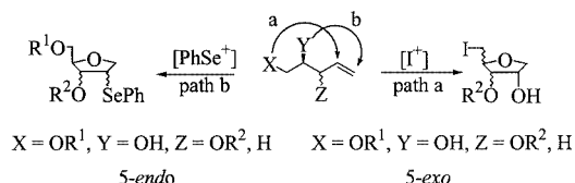
Scheme 2. Chemo- and regioselectivity in the electrophilically induced cyclization of 4-pentene-1,2-diols
