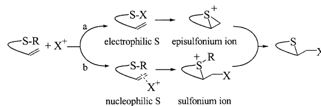
Scheme 1. Proposed mechanisms for the electrophilically induced cyclization of sulfanylalkenes
