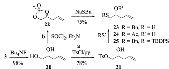
Scheme 6. Synthesis of 1-sulfanyl-4-pentene-2-ol derivatives
