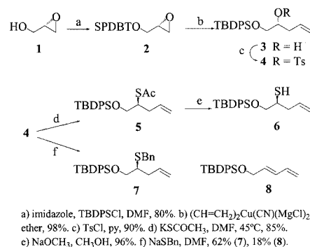
Scheme 3. Synthesis of 2-sulfanyl-4-penten-1-ol derivatives
