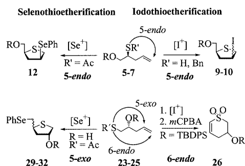
Scheme 9. Summary of the reactivity of 1-sulfanyl- and 2-sulfanylpentenol derivatives towards iodo- and selenothioetherification
